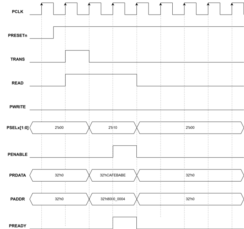
APB Read with Slave 1 access
