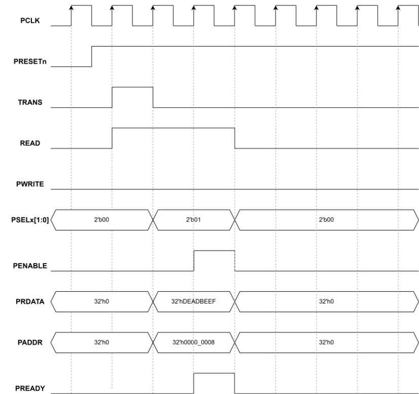
APB Read transfer without waiting state
